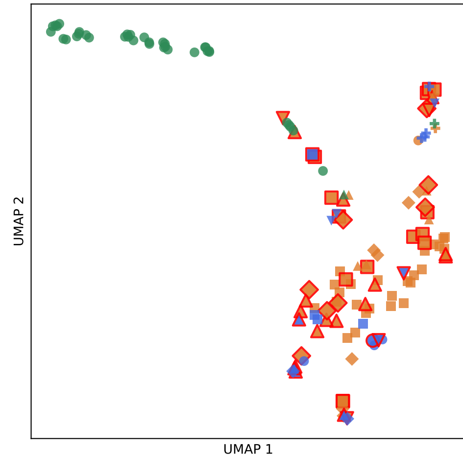
Interaction-trained GCN
