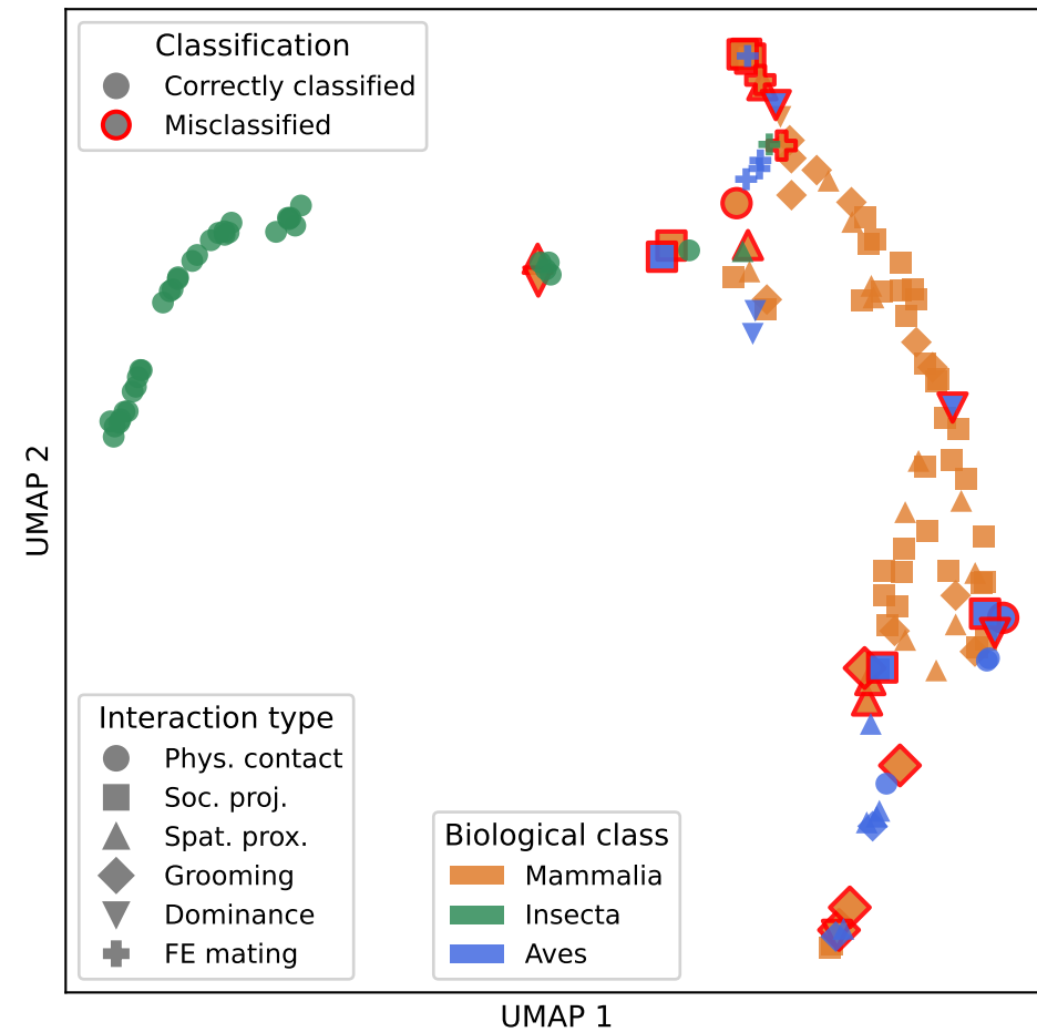
Class-trained GCN
